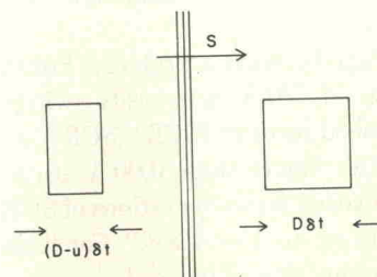
FIG. 5. Geometry for magnetic flux jump condition. Area compression due to shock propagating through magnetic medium at rest is represented. Magnetic field is normal to the page.
